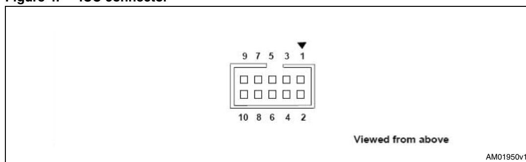
Figure 4. ICC connector
